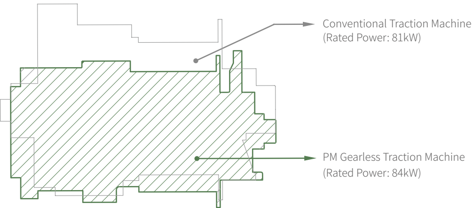
Appearance comparison with conventional Traction Machine This machine is applied to the elevator with capacity 2000kg and speed 480m/min
